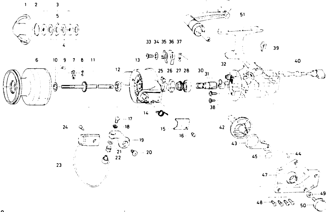
Key No. 2-9 6-L03-0901 Spool assembly
